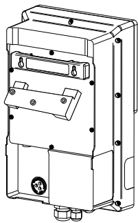
Wall-mounting the equipment
