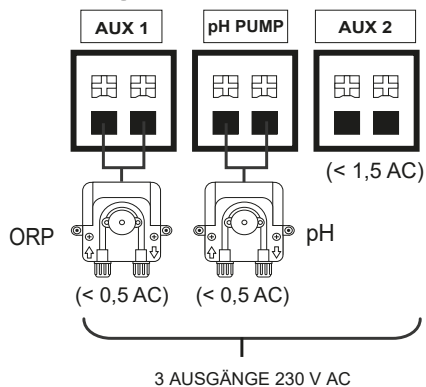
② pH-/ORP-Pumpe
