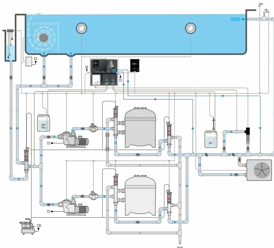
DUAL PUMP SET UP WITH DATA AQUISITION - SALT DISINFECTION - ADDITIONAL CONTROL
