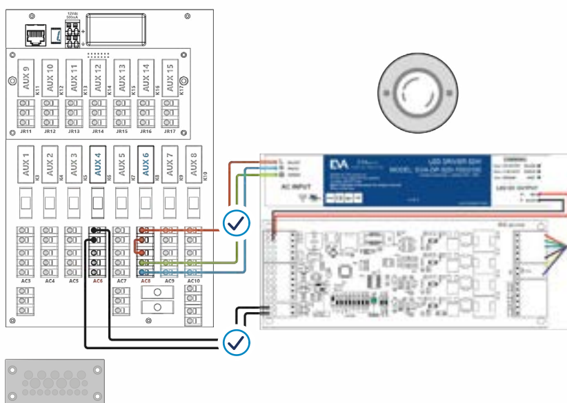
WIRING EXAMPLE FOR EVA OPTIC LIGHTS
