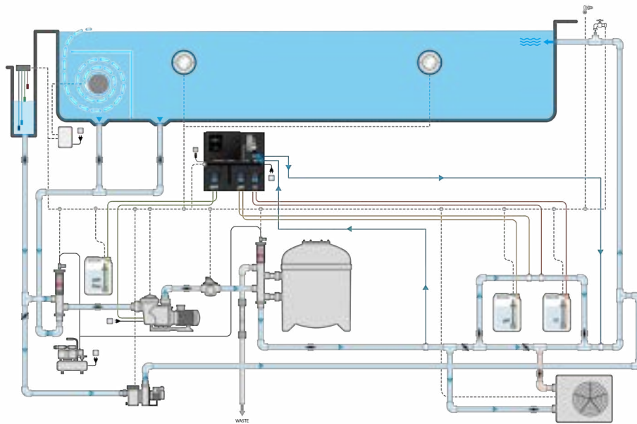
SINGLE PUMP SET UP WITH DATA AQUISITION - CHLORINE DISINFECTION - ADDITIONAL CONTROL
