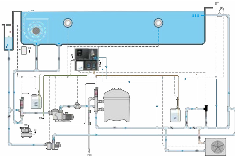
SINGLE PUMP SET UP WITH DATA AQUISITION - SALT DISINFECTION - ADDITIONAL CONTROL
