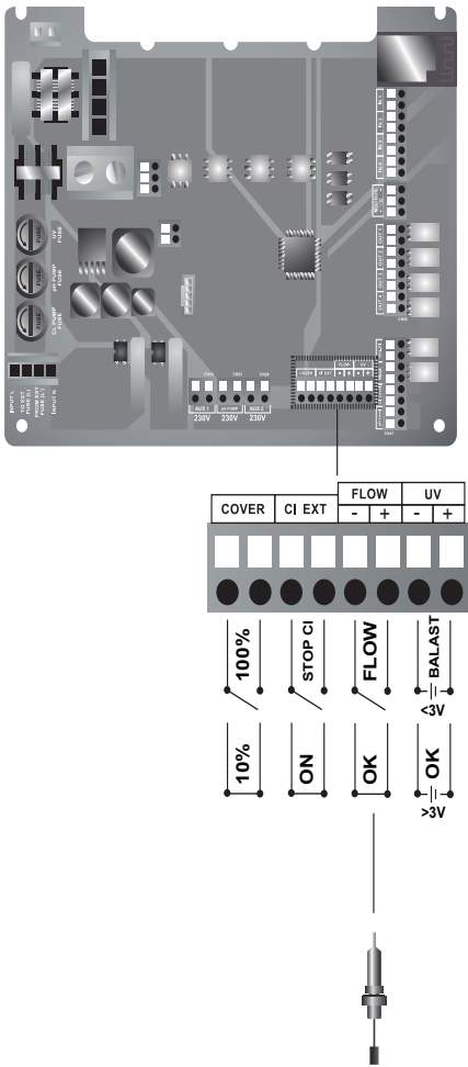
Connecting the flow switch sensor to the main board
