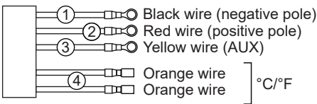
Connecting the gas flow sensor to the device
