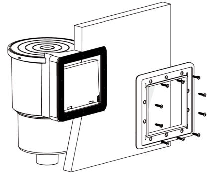
Installing the Skimmer's First Gasket
