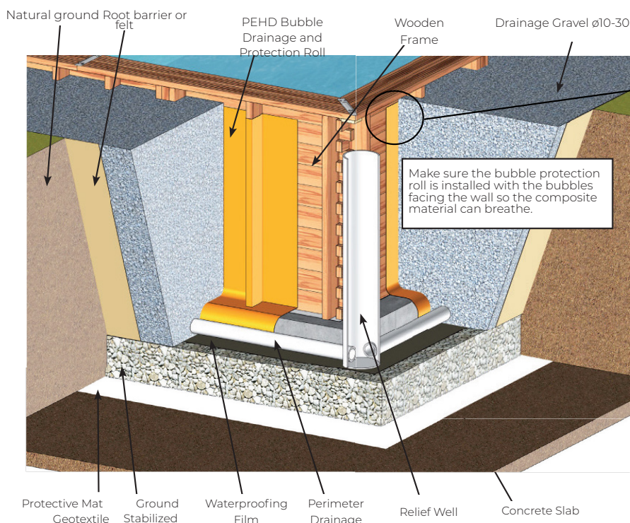
1- Wooden frame 2- PEHD dimpled protection and drainage mat
