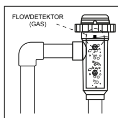
ANBEFALET INSTALLATION
