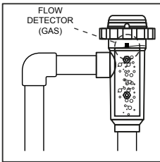
RECOMMENDED installation
