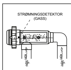
AKSEPTABEL installasjon (along with flow switch installation)
