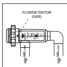
ACCEPTABEL installation (inkl. installation af vandflowskift)
