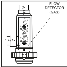
UNACCEPTABLE installation
