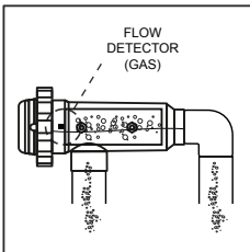
ACCEPTABLE installation (along with flow switch installation)
