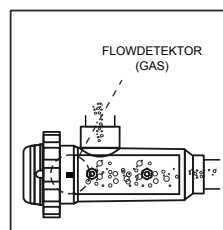
UACCEPTABEL INSTALLATION
