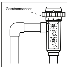
EMPFOHLENE Installation
