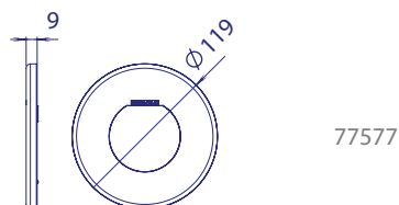
FlexiMini Pure Decorative Ring for liner pools
