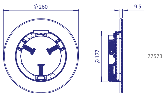
FlexiPure Decorative Ring for liner pools and existing concrete pools
