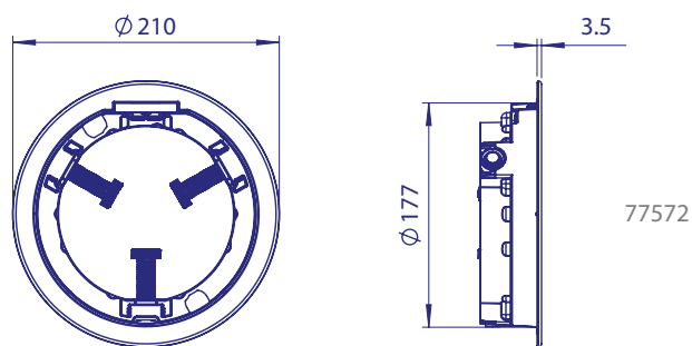
FlexiPure Decorative Ring for concrete pools
